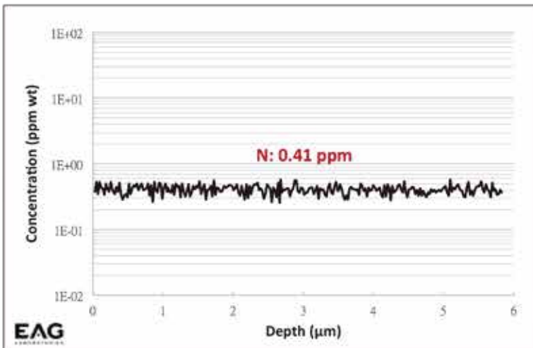
N Concentration in SiC Powder Analysis Using SIMS
