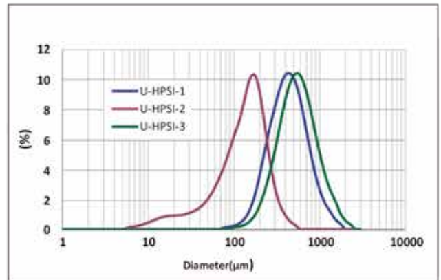
SiC Powder Particle Distribution
